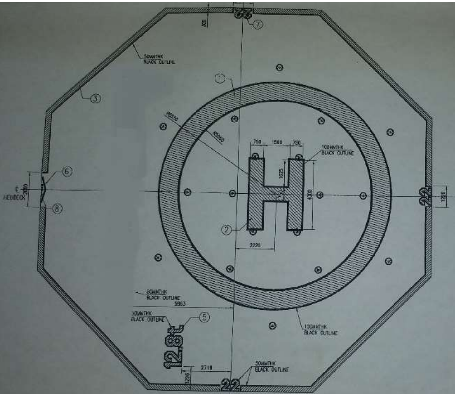
MARKING LAYOUT
