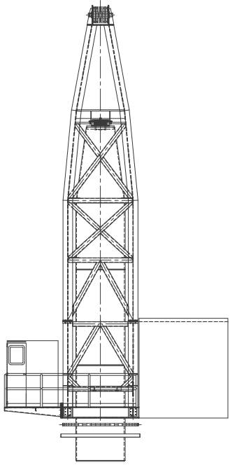
REAR VIEW SCALE: 1/16"=1'-0"
